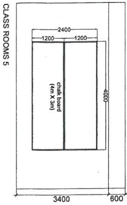
CLASS ROOM-5 PLAN
