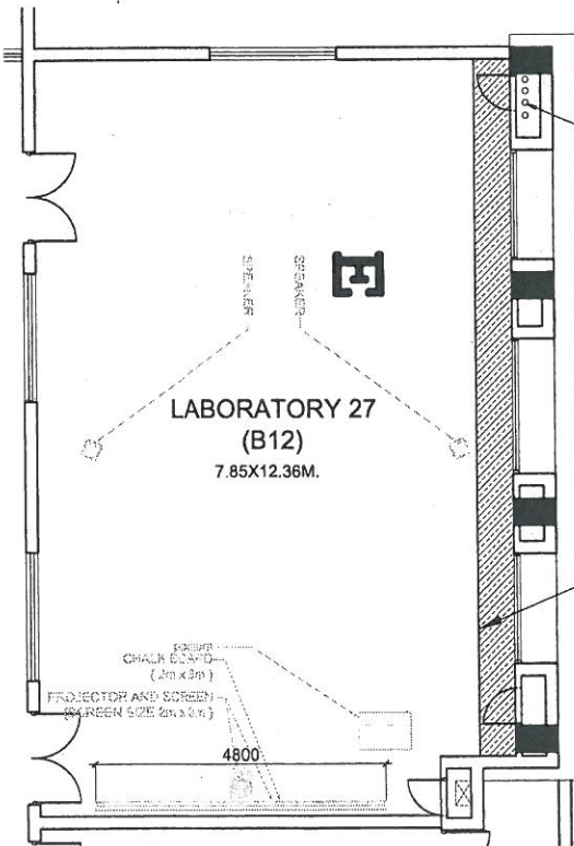
LABORATORY 27 PLAN
